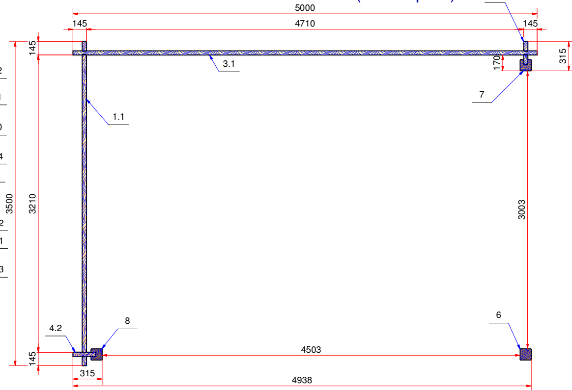
Plan huschen (house plan)
